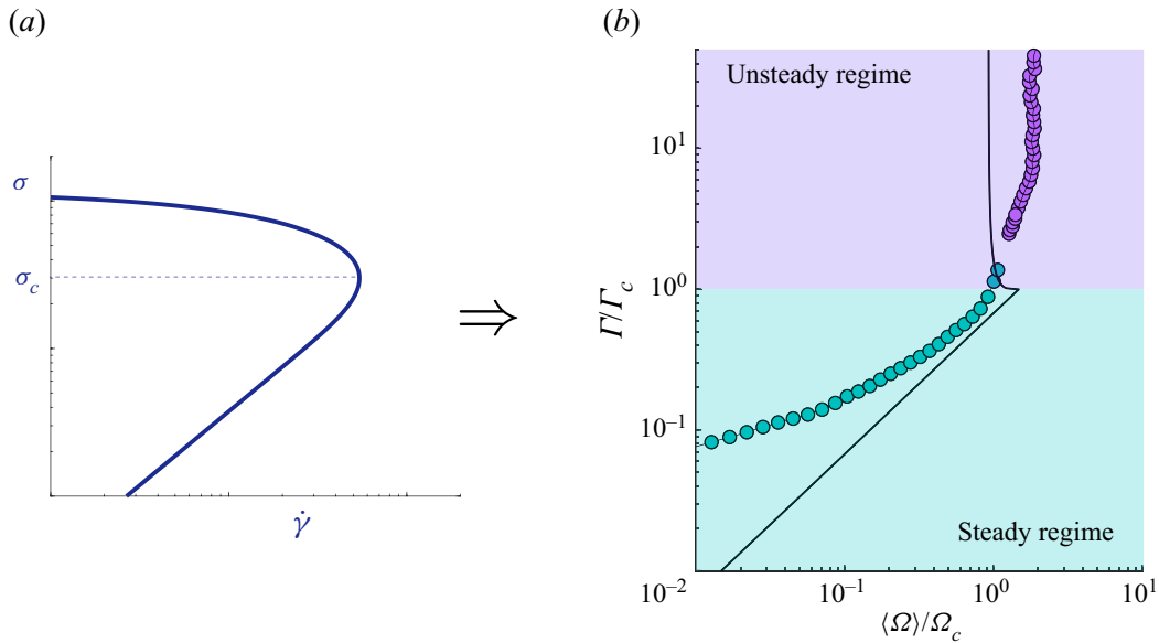
Figure 9. Effective drag of the suspension. (a) The local rheological flow rule is strongly re-entrant for \sigma > \sigma_c . (b) The average cylinder velocity, \langle\Omega\rangle , is marginally re-entrant for \Gamma > \Gamma_c : it essentially saturates at a value of order \Omega_c \approx \dot{\gamma}_c/2 because of the periodic instability of the suspension flow. Solid line: average velocity, \tau^{-1} \int_0^\tau \Omega(t) dt , expected from (3.3) with \Omega_{rel} = \Omega_c/4 (i.e. t' = (I/4\pi\eta_0 hR^2) \ln(1 - \Gamma_c/4\Gamma) ). Symbols: measurements obtained for an increasing ramp of applied torque (short-time averaging of the data of figure 3(a)).
