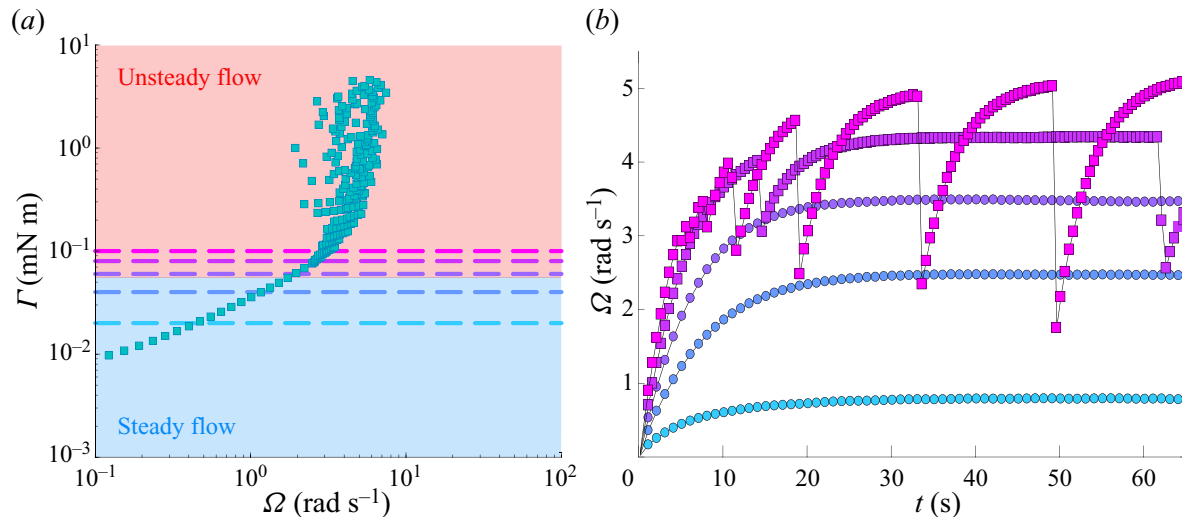
Figure 3. The two regimes of cylinder motion ( \phi = 0.44 > \phi_{DST} ). (a) Applied torque vs angular velocity of the cylinder for a slowly increasing ramp of applied torque ( h = 15 mm). (b) Time evolution of the cylinder speed for constant torques applied at t = 0 s ( \Gamma/\Gamma_c = 0.36, 0.72, 1.07, 1.43 and 1.79 , highlighted by dashed lines in (a)). See also supplementary movie 1.
